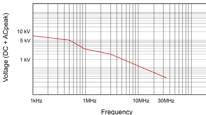
Figure 2: CT4076 Voltage Derating Curve
